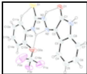
Fig. 1. View of the title compound with the atom numbering scheme. The thermal displacements are drawn at the 30% probability level. The dotted lines indicate the intra-molecular H-bondings. Only the majority group of disordered atoms are shown for clarity.
