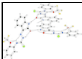
Fig. 2. The partial packing ( PLATON ; Spek, 2009) which shows that molecules form polymeric chains with different ring motifs.
