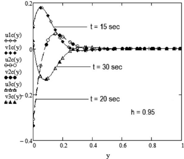
Fig. 8. Profile of velocities u_c(y, 0, t) given by (30a)-curve u_{1c}(y) , u_{2c}(y) , u_{3c}(y) , and v_c(y, t) given by (41)-curve v_{1c}(y) , v_{2c}(y) , v_{3c}(y) for f = 50 , \nu = 0.024 , \mu = 2.28 , \lambda = 1.2 , \lambda_r = 0.8 , \omega = 4 , and different values of t .
