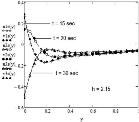
Fig. 7. Profile of velocities u_s(y, 0, t) given by (30b)-curve u_{1s}(y) , u_{2s}(y) , u_{3s}(y) , and v_s(y, t) given by (42)-curve v_{1s}(y) , v_{2s}(y) , v_{3s}(y) for f = 50 , \nu = 0.024 , \mu = 2.28 , \lambda = 1.2 , \lambda_r = 0.8 , \omega = 4 , and different values of t .
