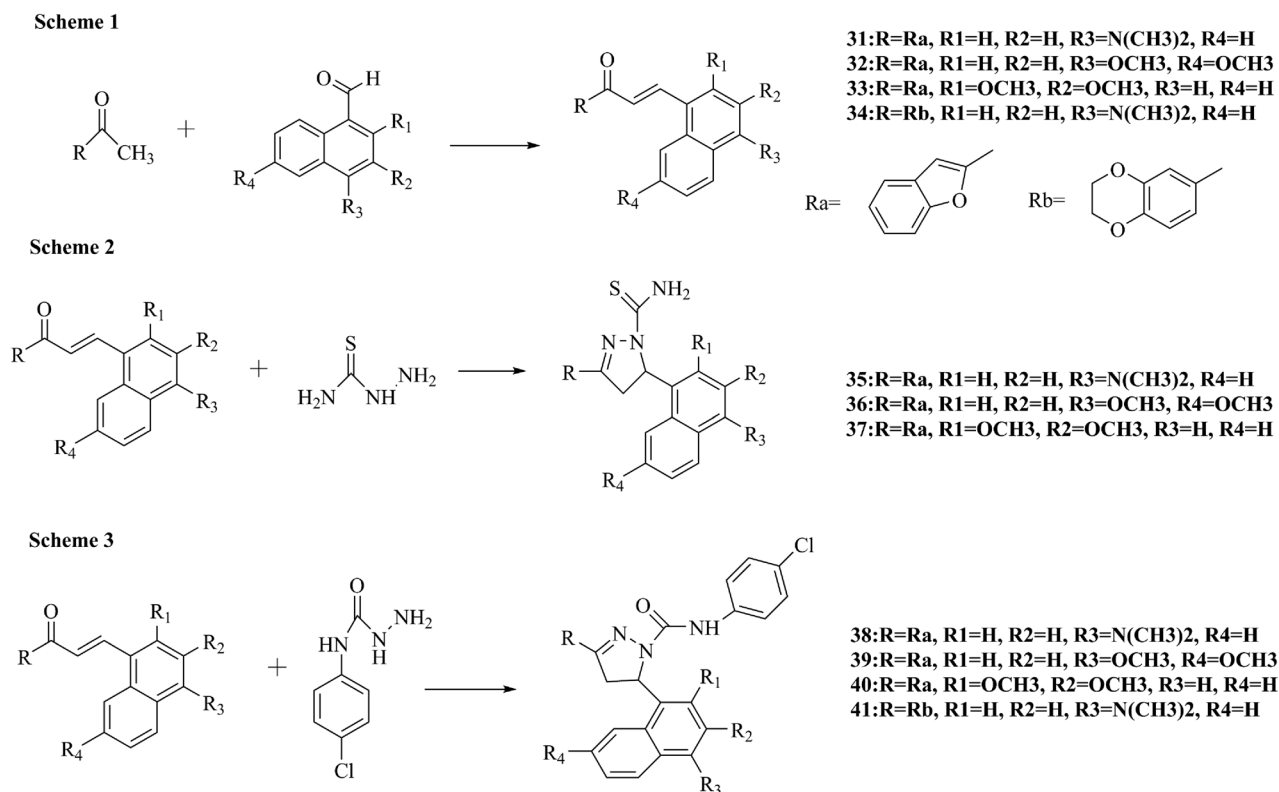
Fig. 2 Structures and synthesis of chalcone derivatives (scheme 1) and pyrazoline derivatives (scheme 2, 3). Reprinted from the Chemical Biology and Drug Design (Bukhari et al. 2015a, 2015b)
